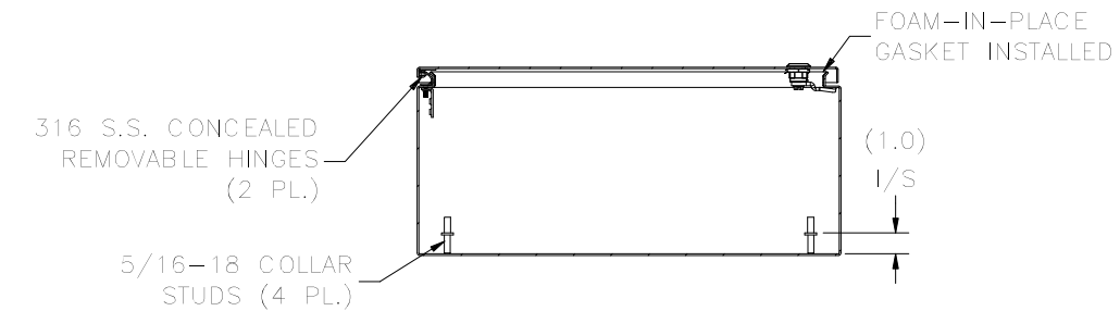
SECTION B-B VIEW (INSIDE TOP OF ENCL.)
