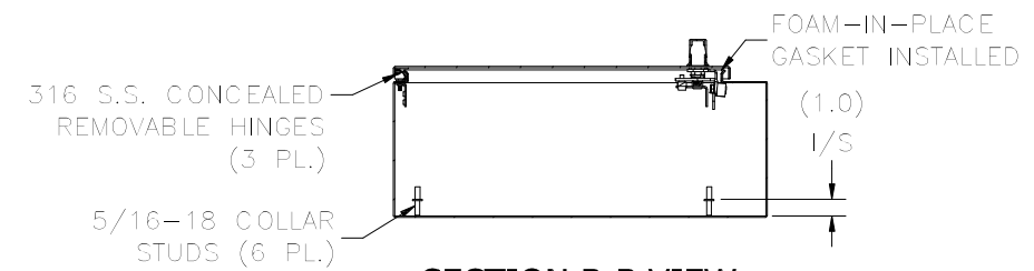
SECTION B-B VIEW (INSIDE TOP OF ENCL.)
