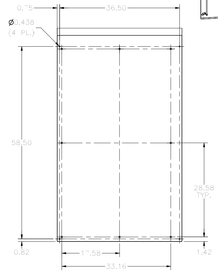
SECTION A-A VIEW (INSIDE BACK OF ENCL.)
