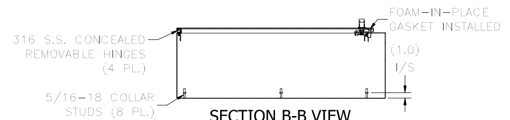
SECTION B-B VIEW (INSIDE TOP OF ENCL.)
