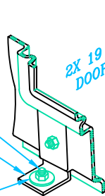
ENCLOSURE BOLT DOWN DETAIL
