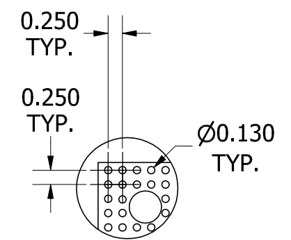
DETAIL-A (PERFORATED DETAIL)
