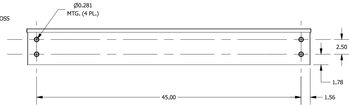
BACK VIEW
