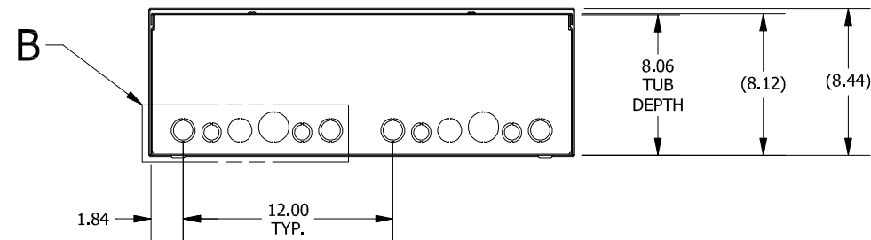
BOTTOM VIEW
