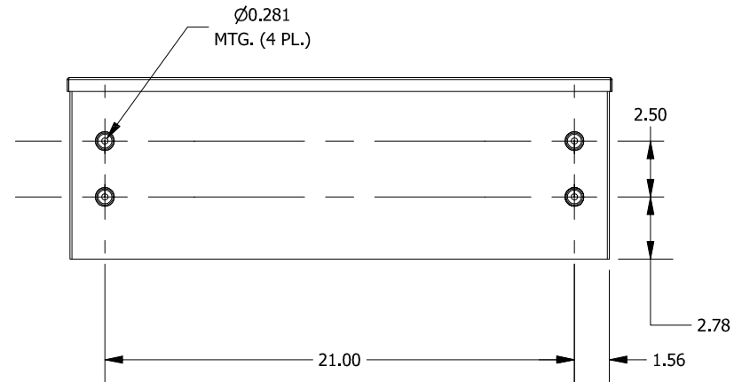
BACK VIEW
