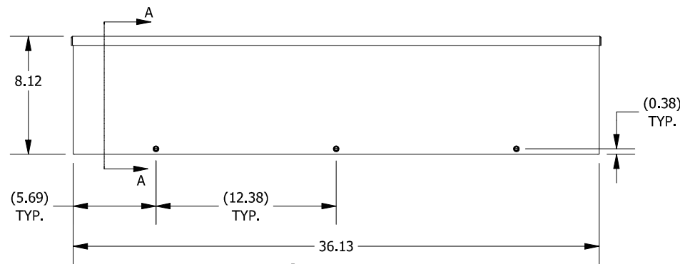
FRONT VIEW
