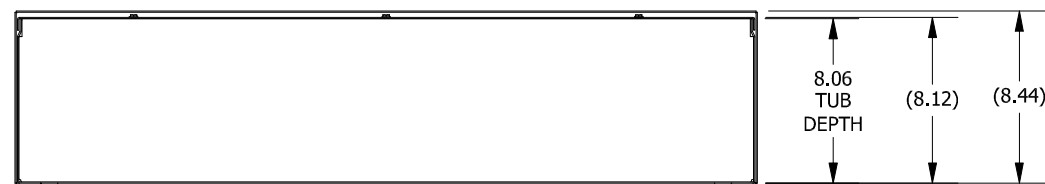
BOTTOM VIEW
