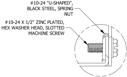
DETAIL A (5 PL.) (LID ATTACHMENT DETAIL)
