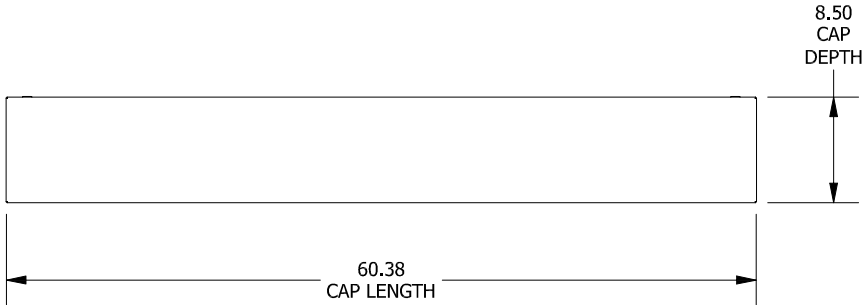
DETAIL A (5 PL.) (LID ATTACHMENT DETAIL)
