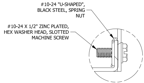
DETAIL A (2 PL.) (LID ATTACHMENT DETAIL)
