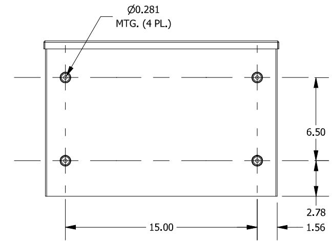
BACK VIEW
