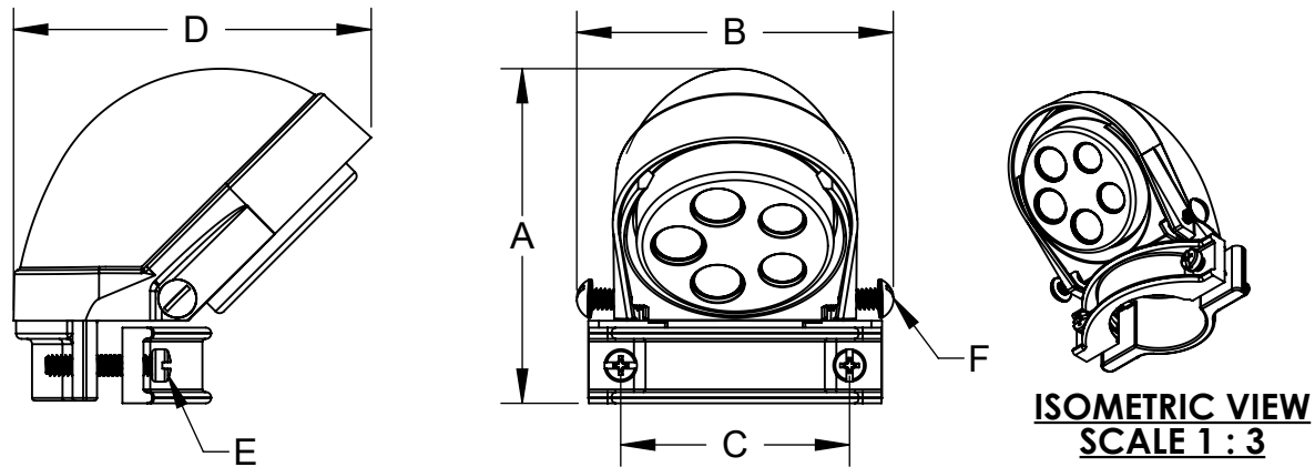
CAT. # 2402 TO 2408
