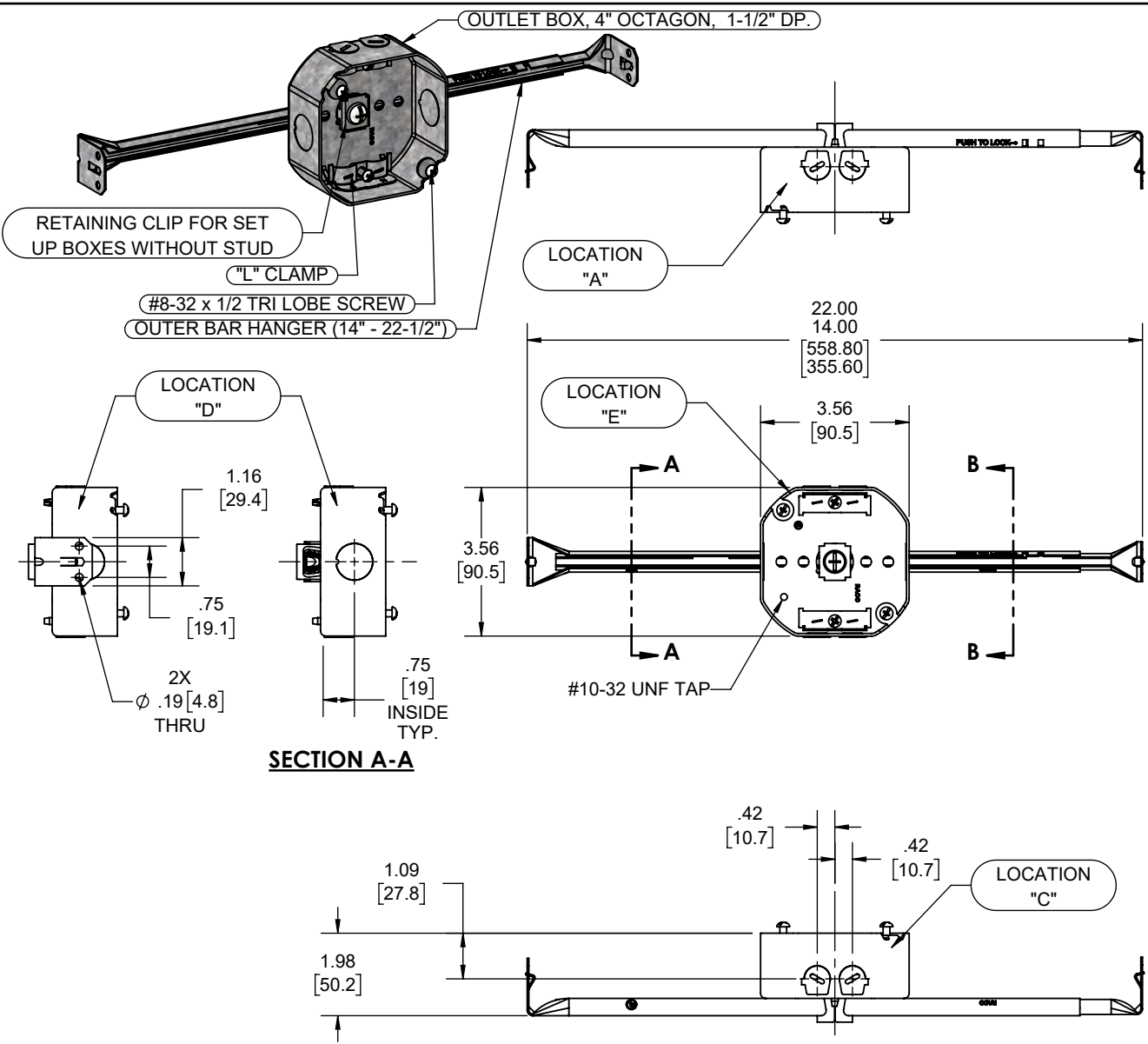
SECTION B-B
