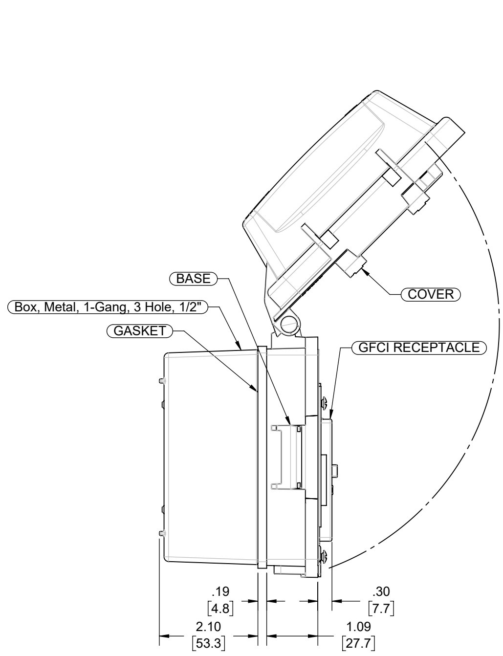
SHOWN OPENED SCALE 1:2
