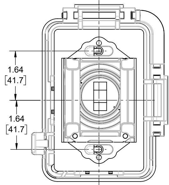
REAR VIEW SCALE 1:2
