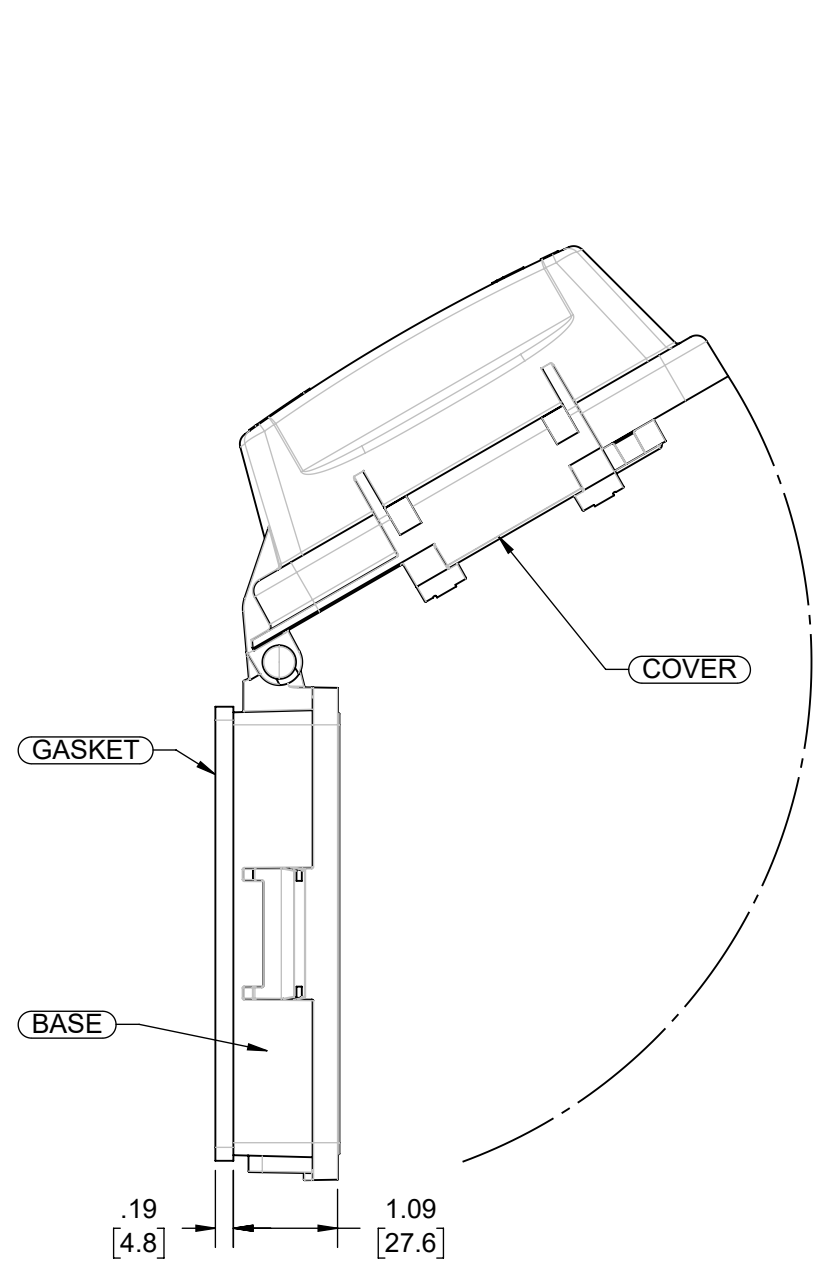
SHOWN OPENED SCALE 1:2
