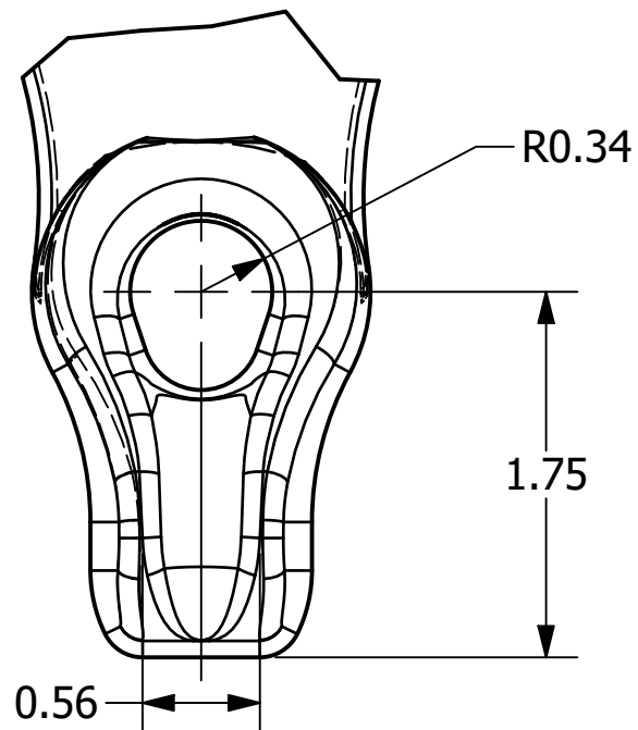
THIMBLEYE DETAIL
