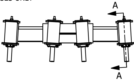
GRILLAGE WITH PILES
