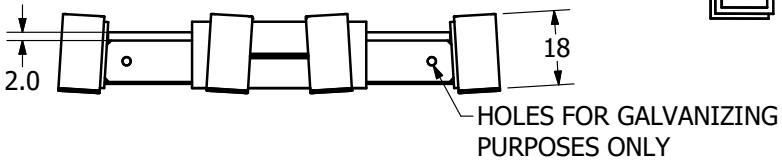
GRILLAGE NO PILES
