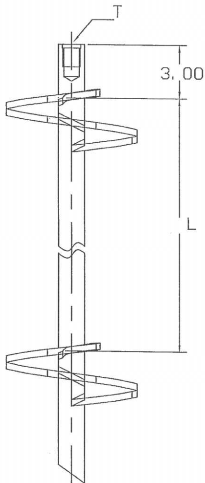
TWIN HELIX ANCHOR WITH SHARPENED LEADING EDGE
