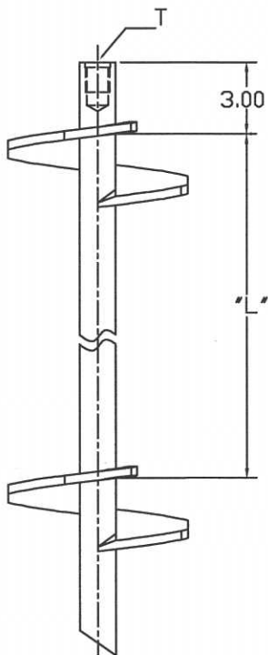
TWIN HELX ANCHDR WITH SHARPENED LEADING EDGE
