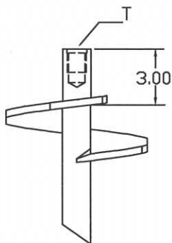
SINGLE HELX ANCHOR WITH SHARPENED LEADING EDGE
