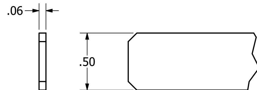
STRAP DETAILS
