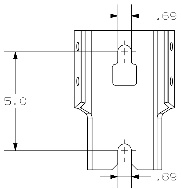
MOUNTING PLATE
