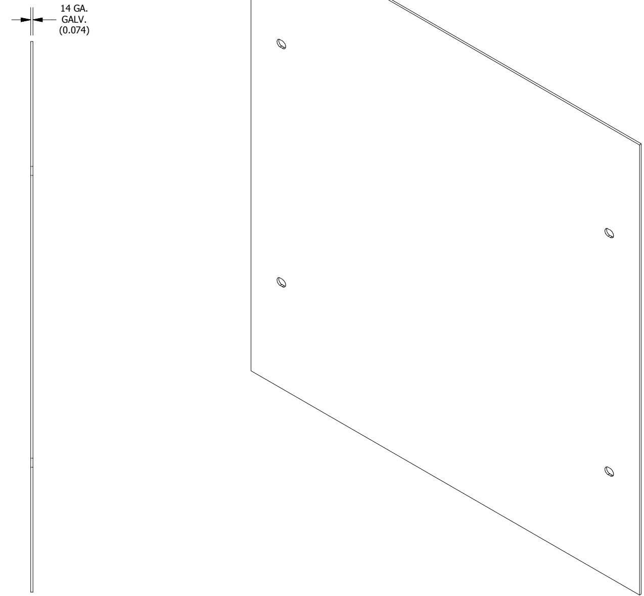
SIDE VIEW
