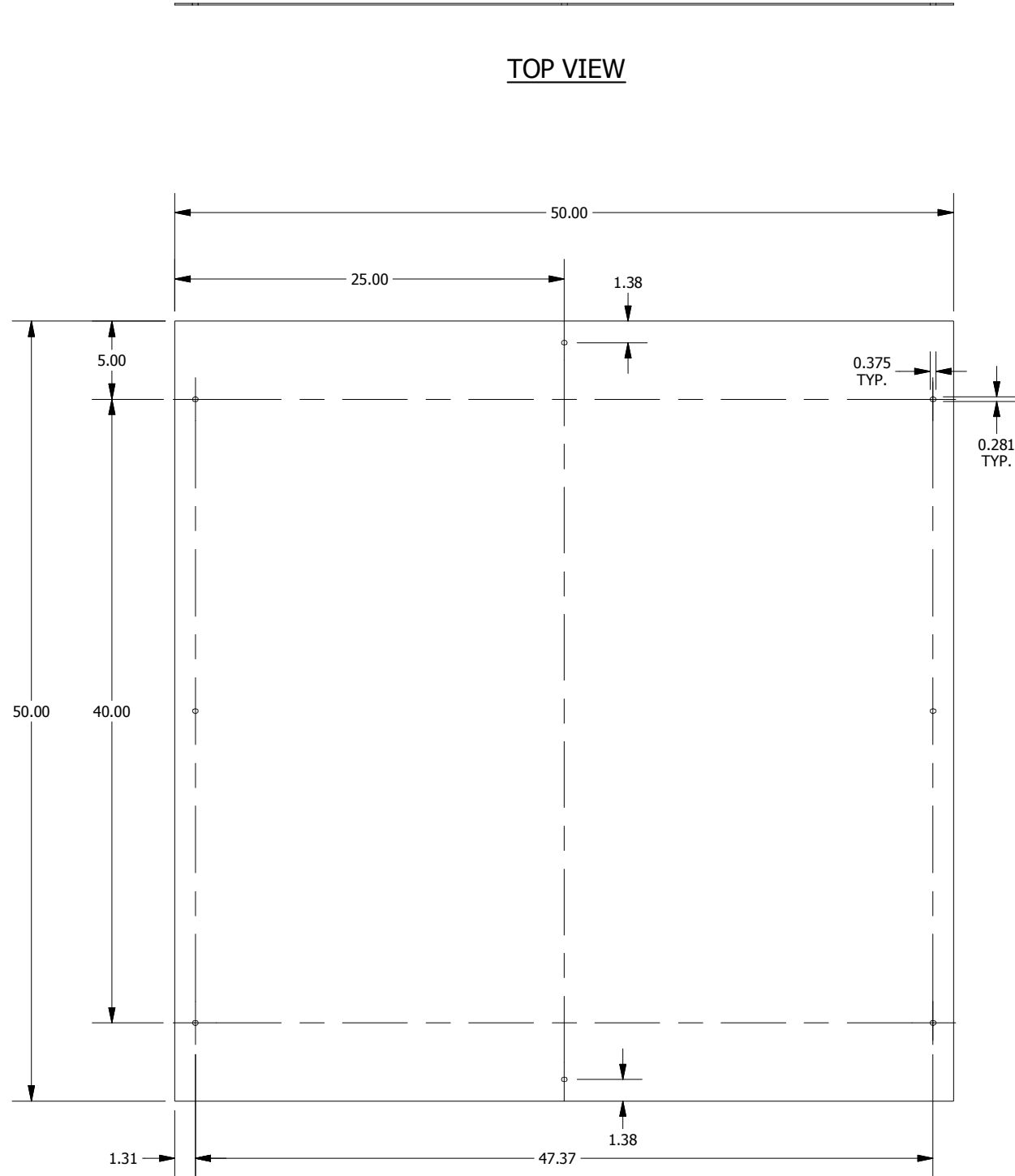
FRONT VIEW
