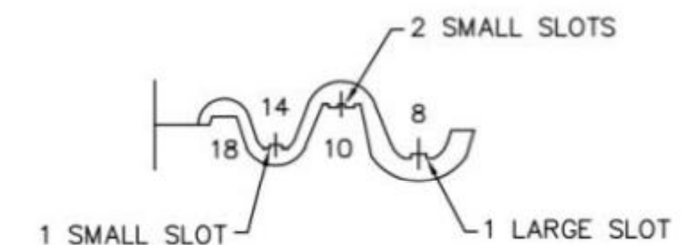
DETAIL A CRIMP GROOVE IDENTIFICATION
