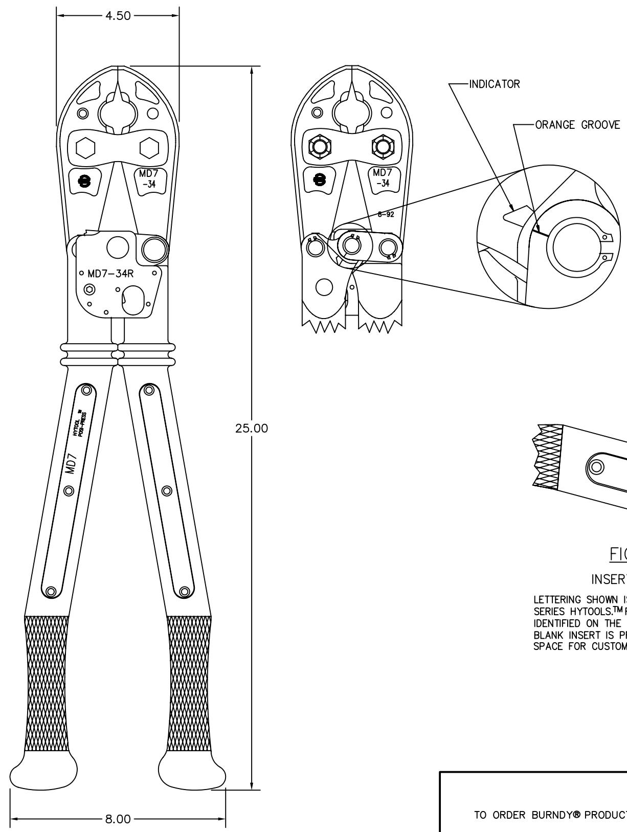
FIGURE 1 MD7-34R POSI-PRESS HYTOOL™
