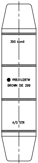
TYPICAL LETTERING VIEW
