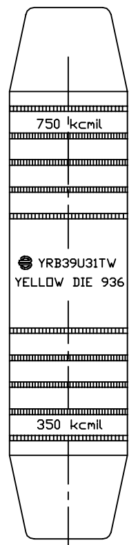
TYPICAL LETTERING VIEW
