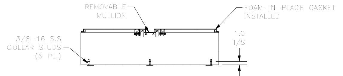
SECTION B-B (INSIDE VIEW OF TOP)
