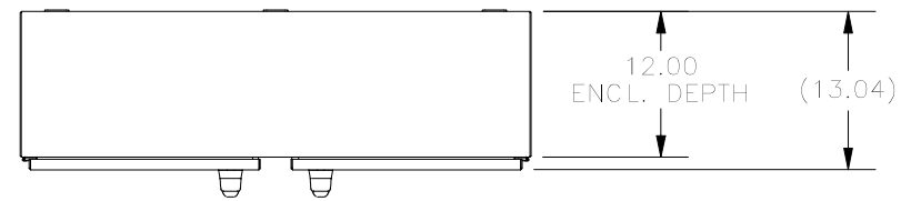
TOP VIEW
