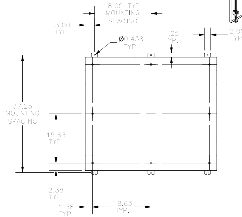
SECTION A-A (INSIDE BACK VIEW OF ENCL.)
