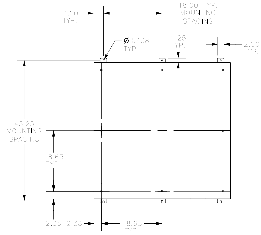
SECTION A-A (INSIDE BACK VIEW OF ENCL.)
