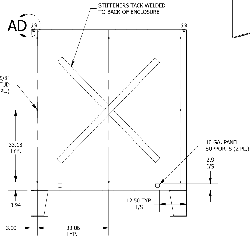
SECTION A-A (INSIDE BACK VIEW OF ENCLOSURE)
