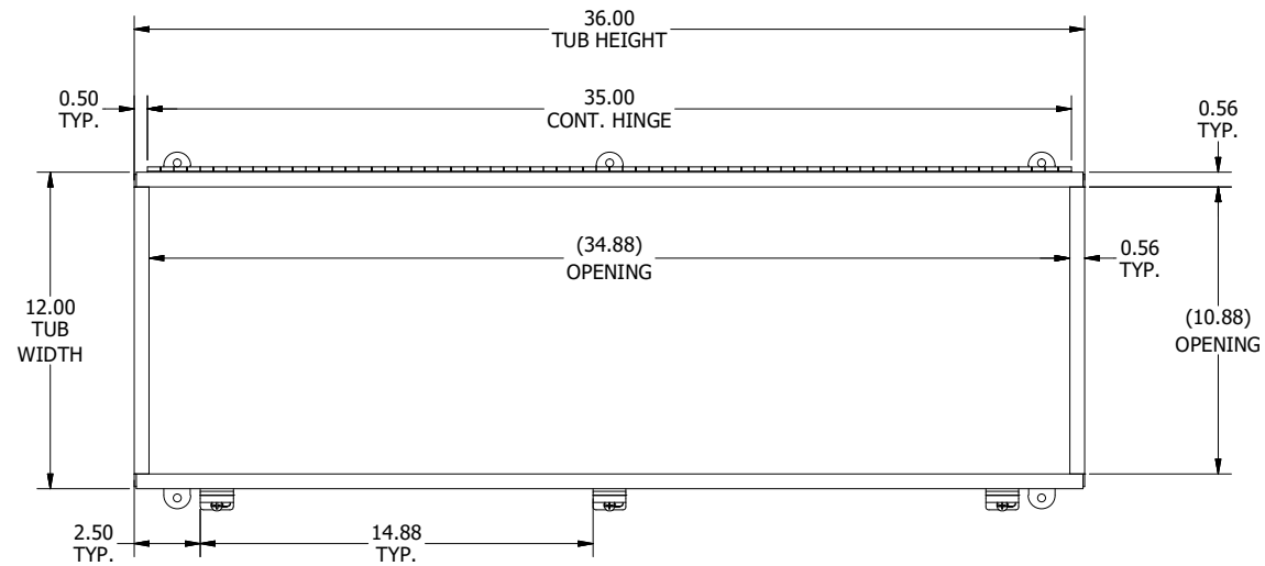
TOP VIEW (COVER REMOVED)
