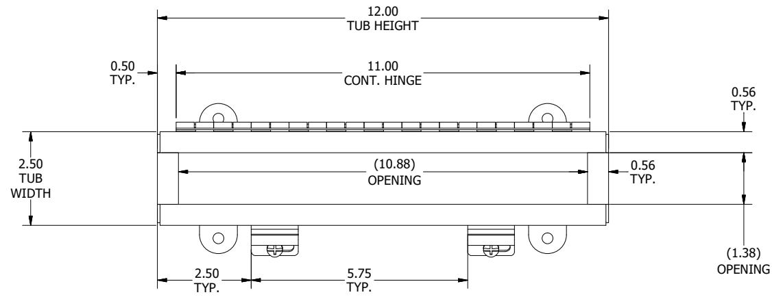
TOP VIEW (COVER REMOVED)
