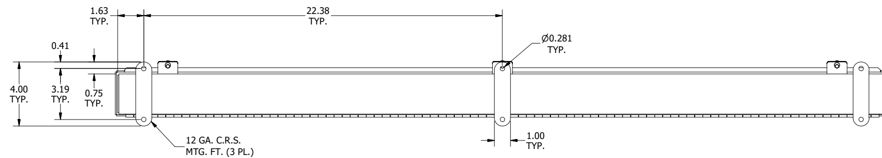
BOTTOM VIEW
