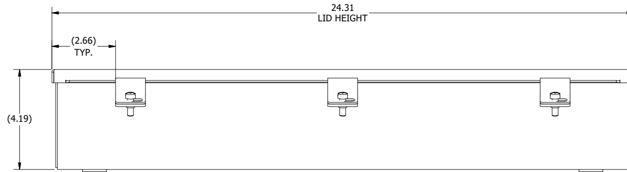
FRONT VIEW
