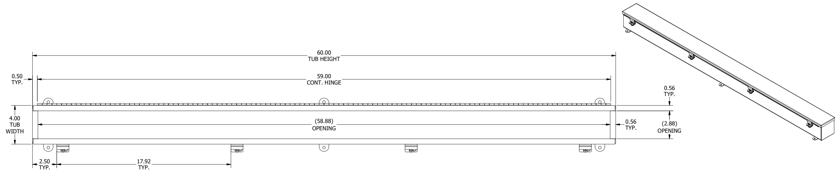
TOP VIEW (COVER REMOVED)
