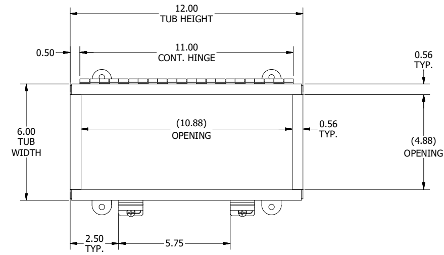
TOP VIEW (COVER REMOVED)
