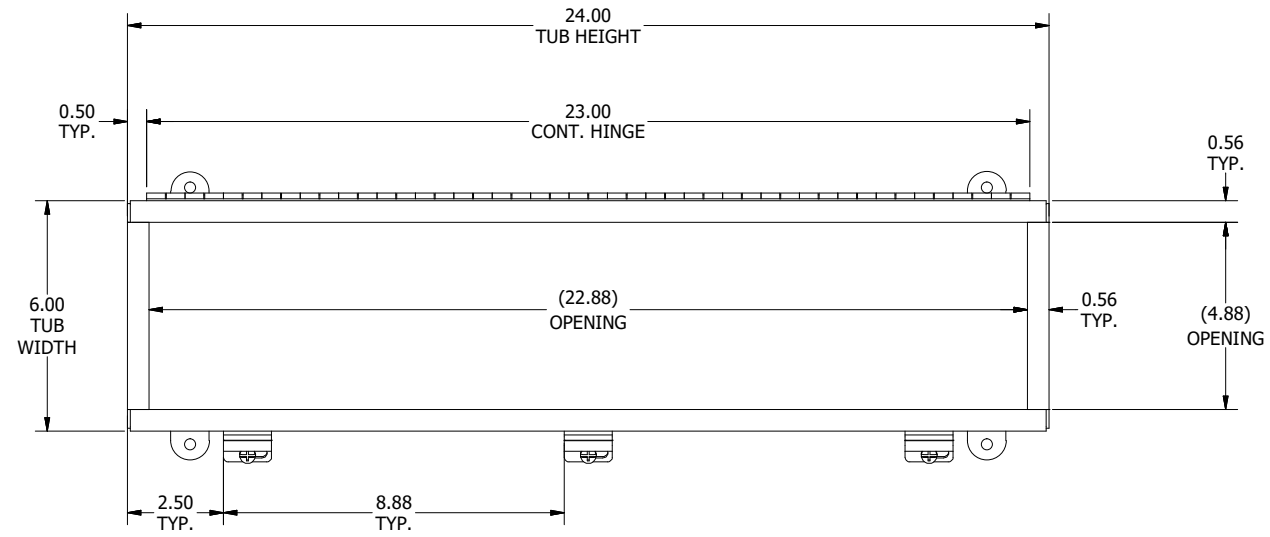
TOP VIEW (COVER REMOVED)
