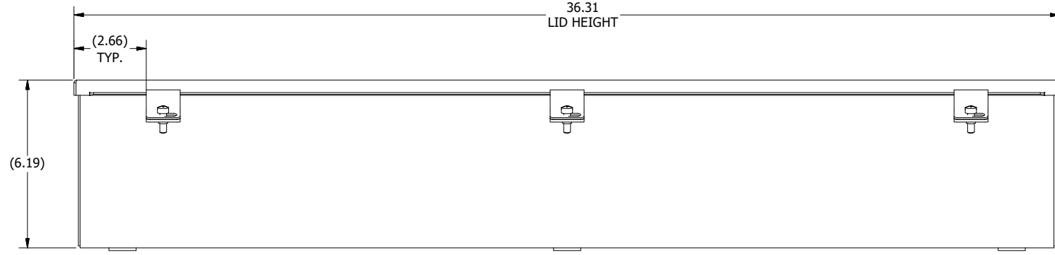
FRONT VIEW
