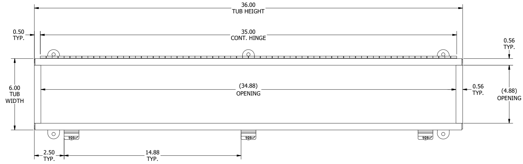
TOP VIEW (COVER REMOVED)
