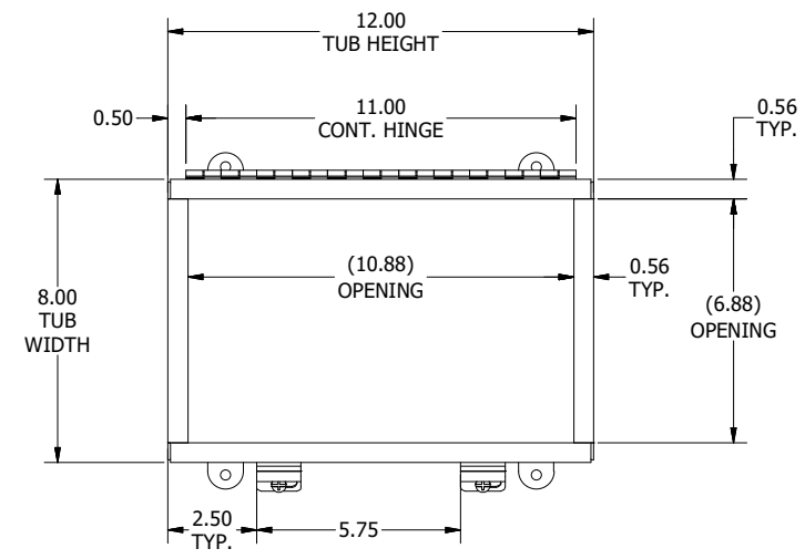
TOP VIEW (COVER REMOVED)
