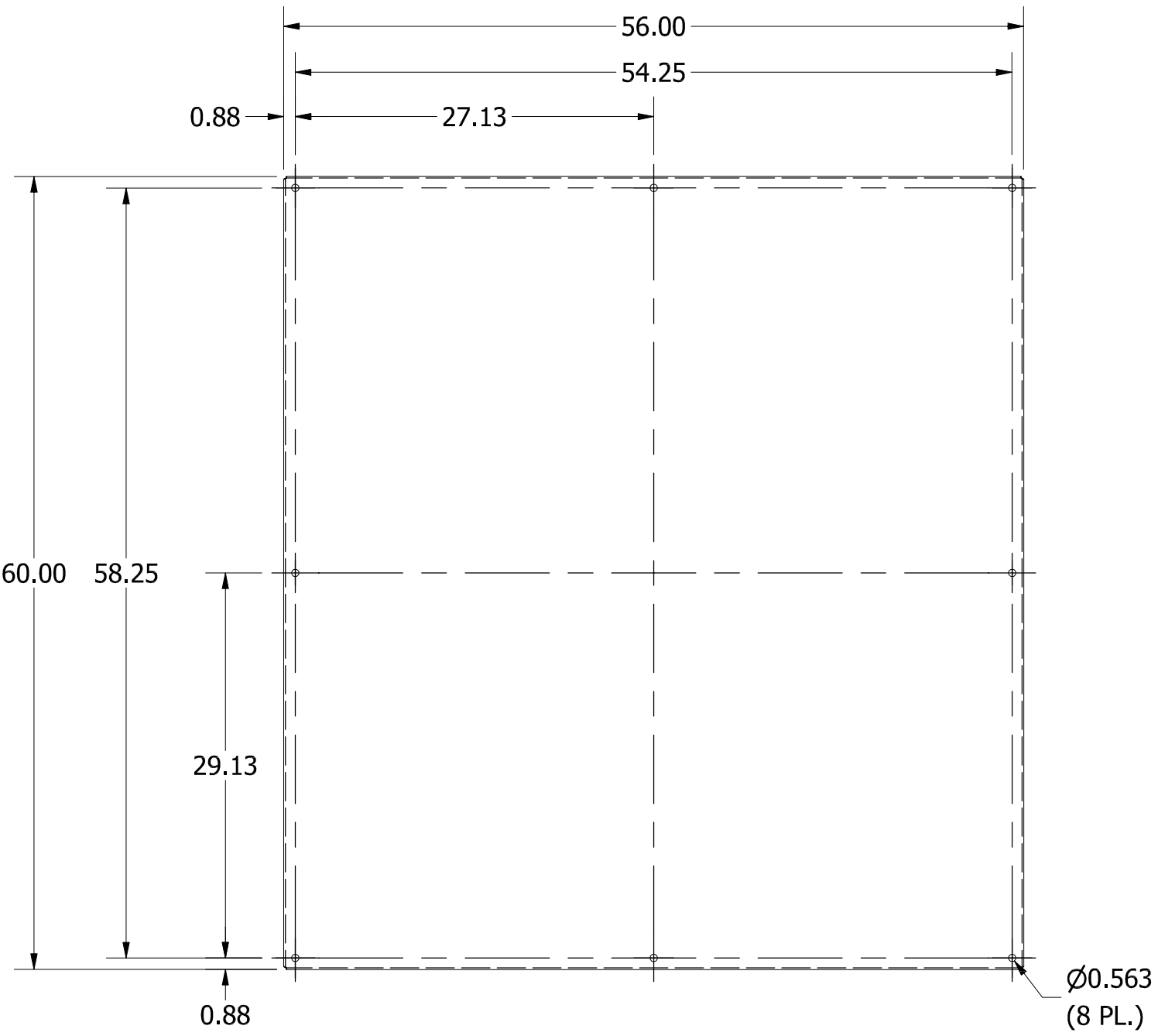
FRONT VIEW
