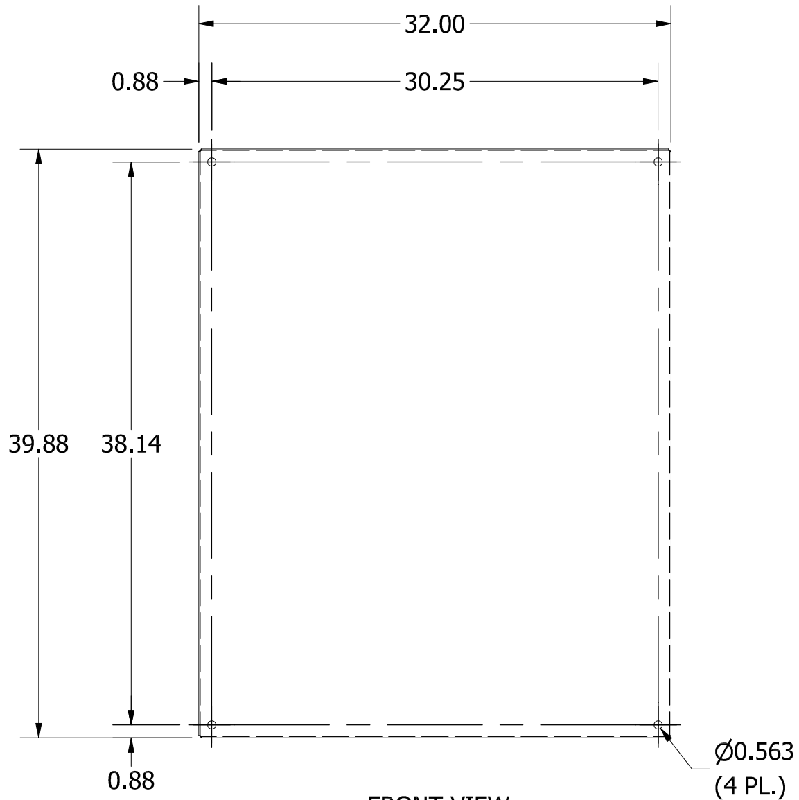
FRONT VIEW
