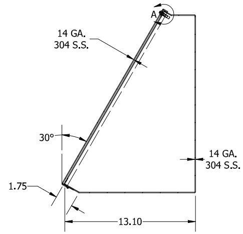
SECTION A-A VIEW (INSIDE LEFT OF ENCL.)
