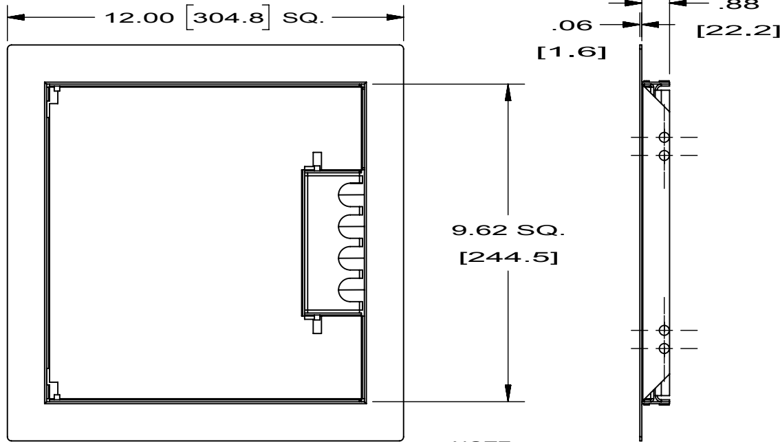
VIEW "A" COVER
