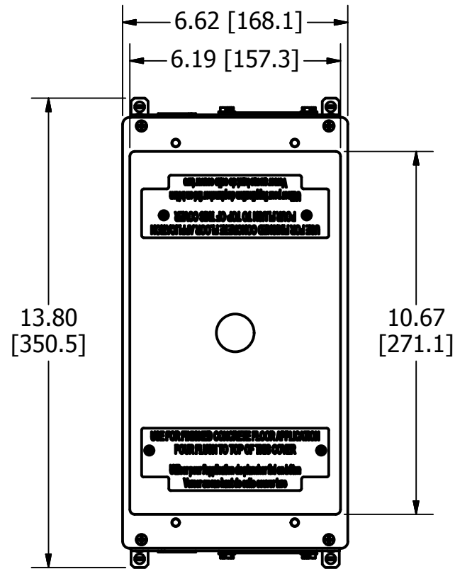
TOP VIEW
