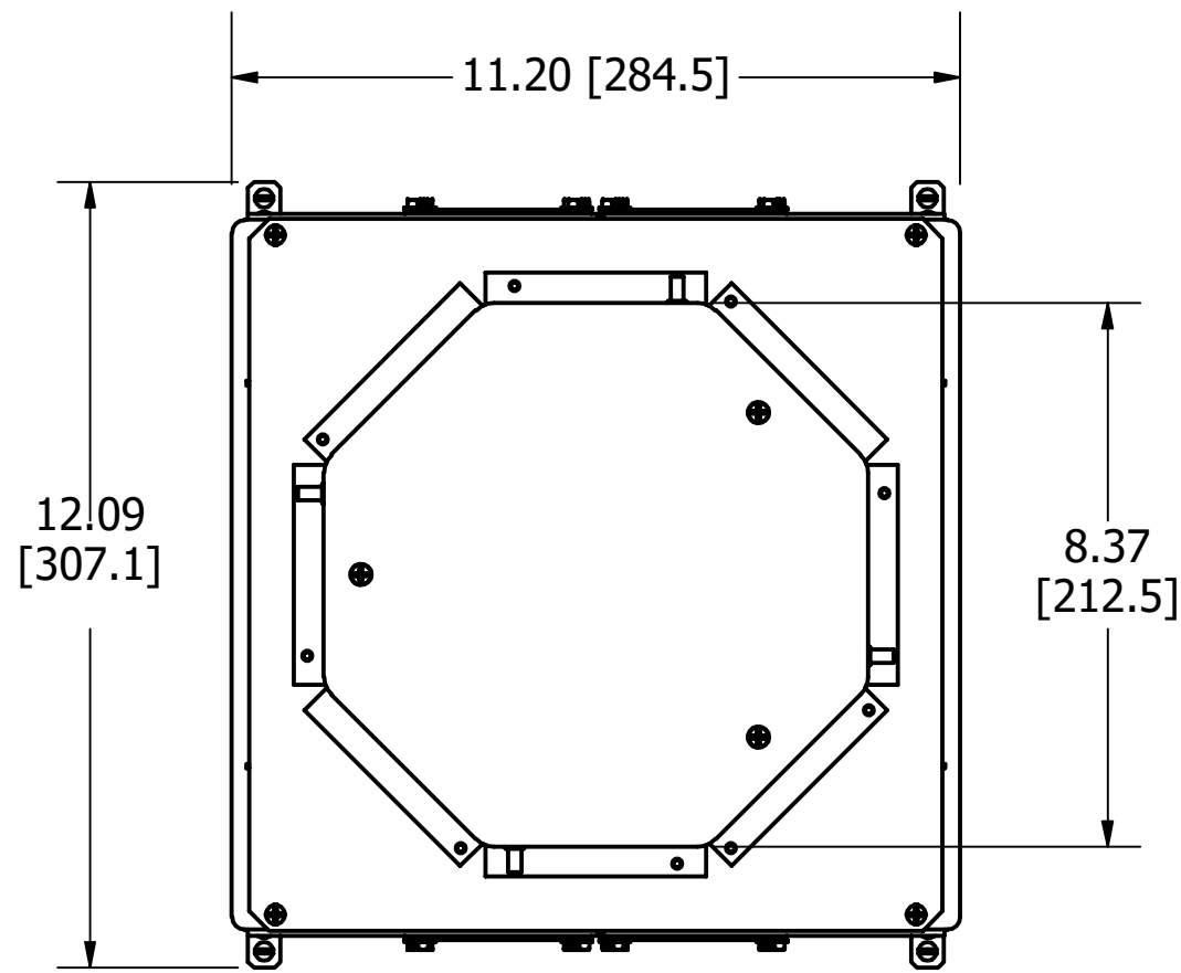
TOP VIEW
