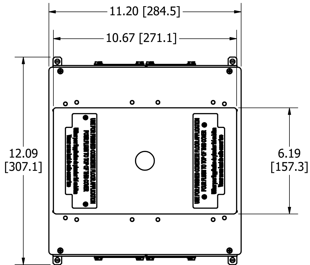
TOP VIEW
