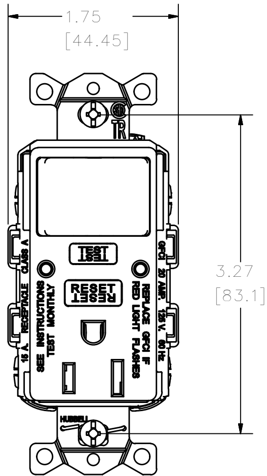
TYPICAL 15A TR DEVICE
