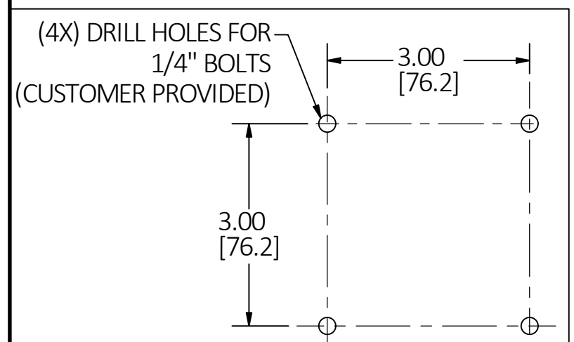
DRILL FOR MOUNTING SCALE 1 / 2
