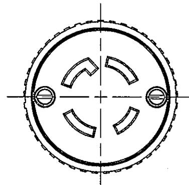
L1430C SHOWN
